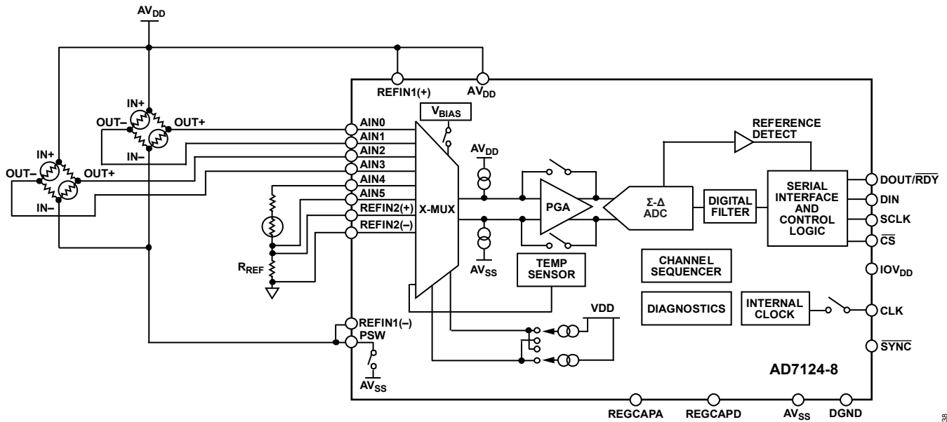
Figure 128. Flowmeter Application
