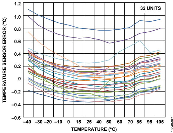
Figure 47. Temperature Sensor Accuracy
