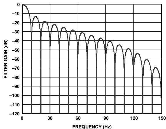
Figure 108. Simultaneous 50 Hz and 60 Hz Rejection
