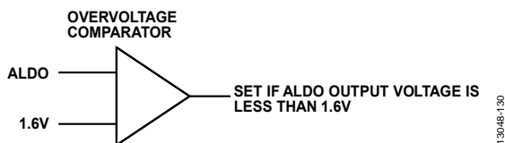
Figure 120. Analog LDO Monitor
