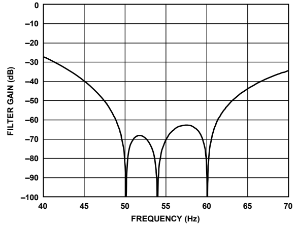
Figure 113. Zoom in 40 Hz to 70 Hz, 25 SPS Output Data Rate, 40 ms Settling Time
