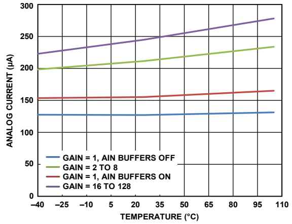
Figure 38. Analog Current vs. Temperature (Low Power Mode)
