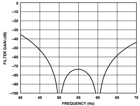
Figure 115. Zoom in 40 Hz to 70 Hz, 20 SPS Output Data Rate, 50 ms Settling Time
