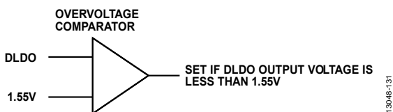
Figure 121. Digital LDO Monitor
