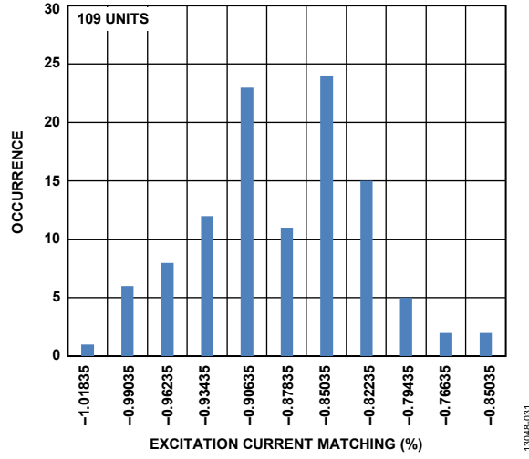
Figure 31. IOUTx Current Initial Matching Histogram (500 μA)
