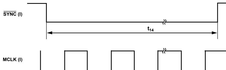
Figure 8. SYNC Pulse Width
