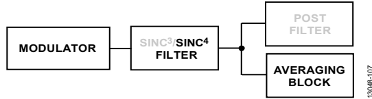
Figure 97. Fast Settling Mode, Sinc 4 + Sinc 1 Filter
