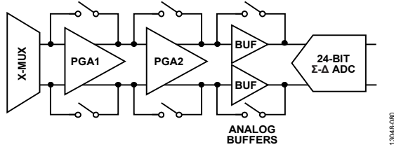
Figure 74. PGA
