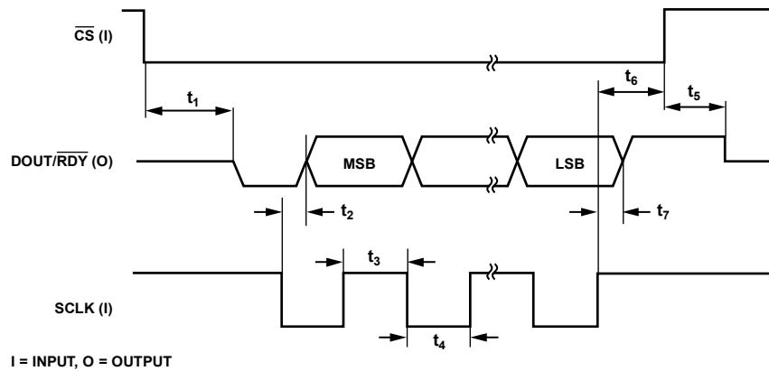
Figure 3. Read Cycle Timing Diagram ( CS\_EN Bit Cleared)
