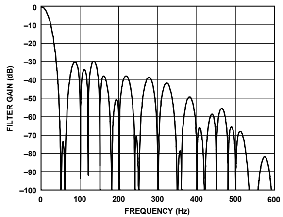
Figure 114. DC to 600 Hz, 20 SPS Output Data Rate, 50 ms Settling Time
