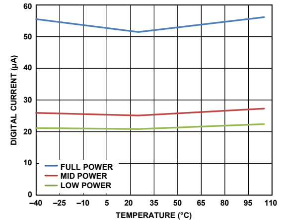
Figure 39. Digital Current vs. Temperature
