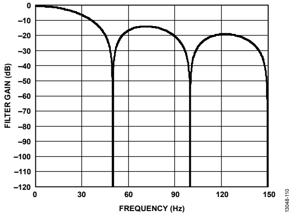
Figure 100. 50 Hz Rejection
