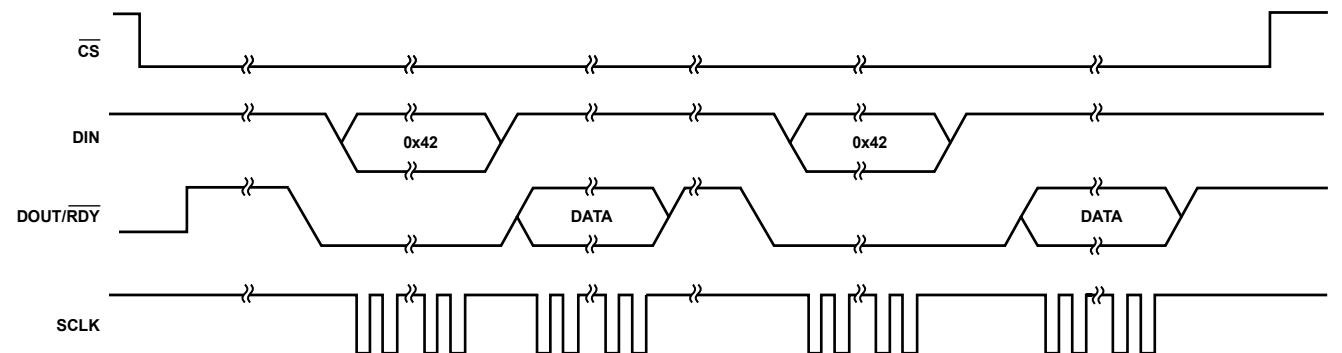
Figure 79. Continuous Conversion Configuration
