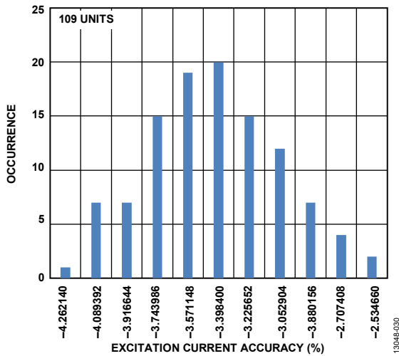
Figure 30. IOUTx Current Initial Accuracy Histogram (500 μA)
