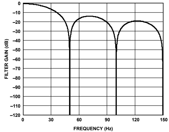
Figure 106. 50 Hz Rejection
