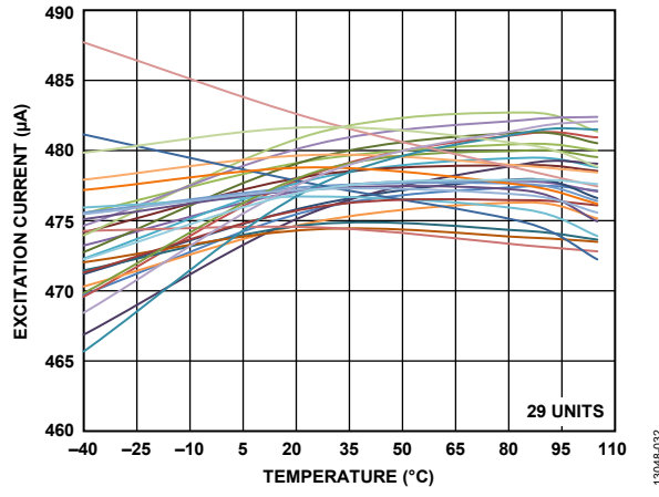
Figure 32. Excitation Current Drift (500 μA)
