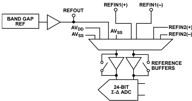
Figure 75. Reference Connections
