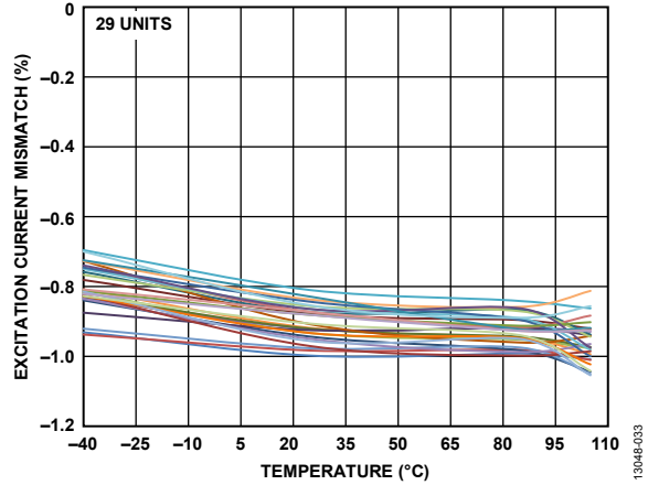
Figure 33. Excitation Current Drift Matching (500 μA)
