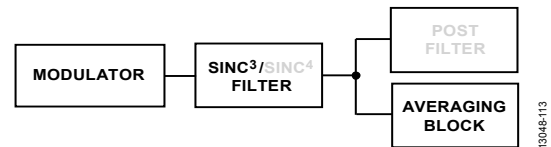
Figure 103. Fast Settling Mode, Sinc 3 + Sinc 1 Filter
