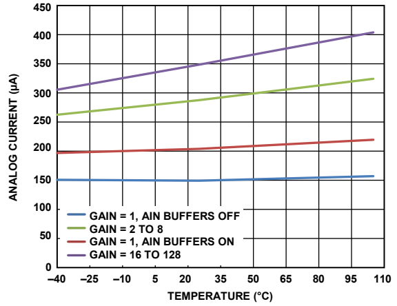
Figure 37. Analog Current vs. Temperature (Mid Power Mode)
