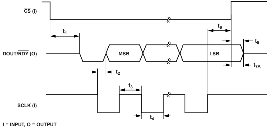
Figure 4. Read Cycle Timing Diagram (CSB_EN Bit Set)
