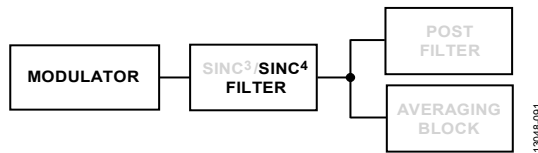
Figure 81. Sinc 4 Filter
