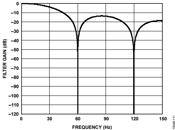
Figure 101. 60 Hz Rejection
