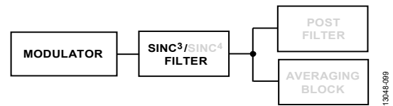
Figure 89. Sinc 3 Filter
