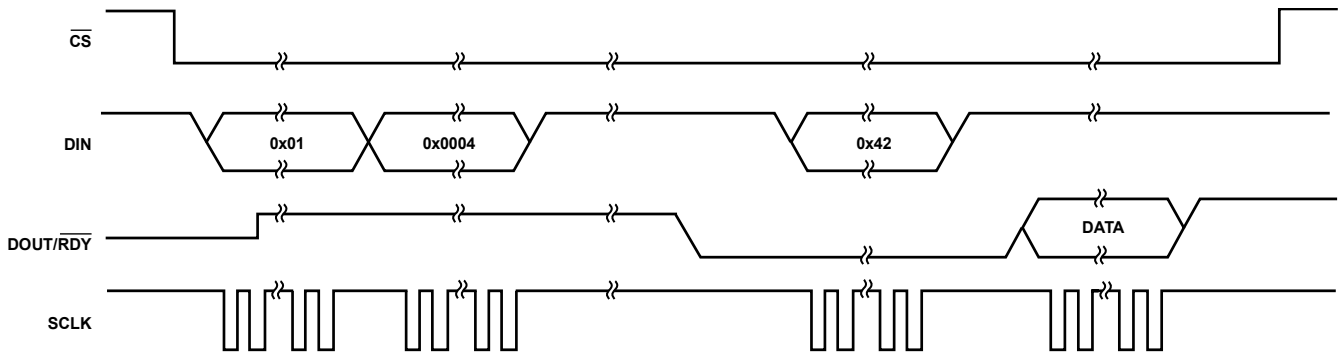
Figure 78. Single Conversion Configuration
