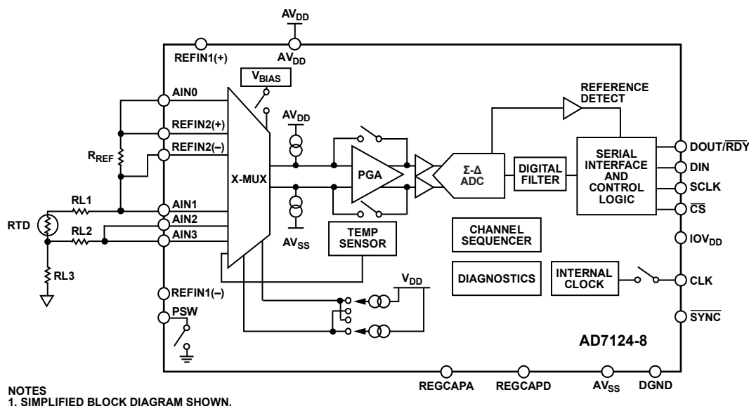
Figure 127. 3-Wire RTD Application
